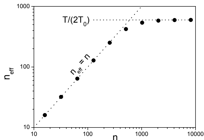
Fig. 3. The function n_{eff} vs. n for the AR(1) model. The parameters of the plot,
